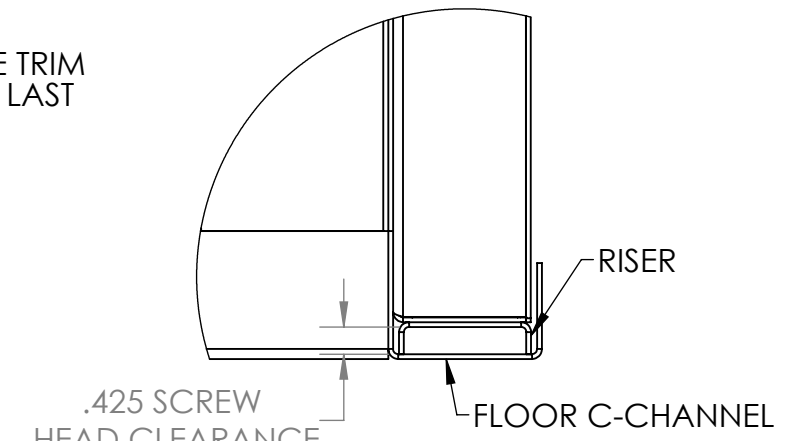
DETAIL B SCALE 1 : 3
