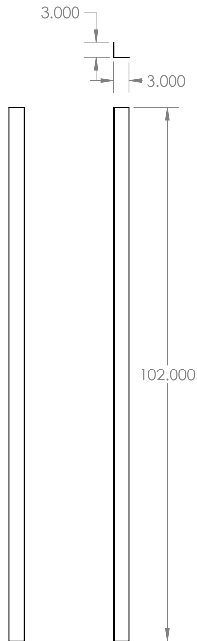
OUTSIDE CORNER TRIM
