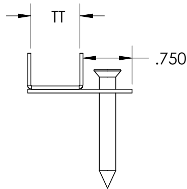
SSUC-SF-LL-TT S/S U-Channel w/ Single Flange
