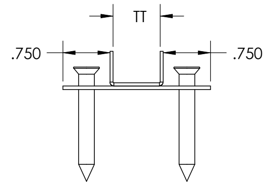
SSUC-DF-LL-TT S/S U-Channel w/ Double Flange
